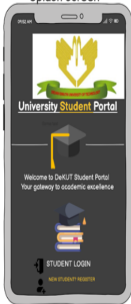
Splash screen
